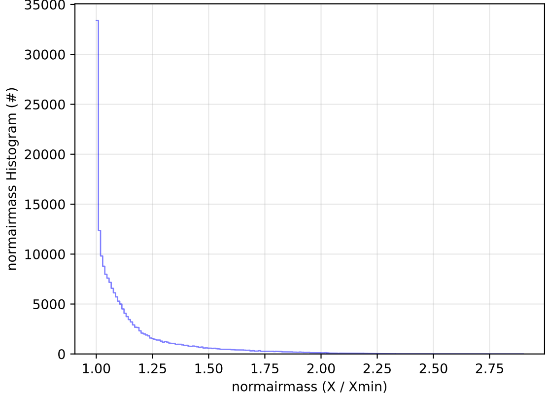
too_elab_2yr_r128_d3_ugrizy_v3.4_10yrs All sky g band: normairmass Histogram
