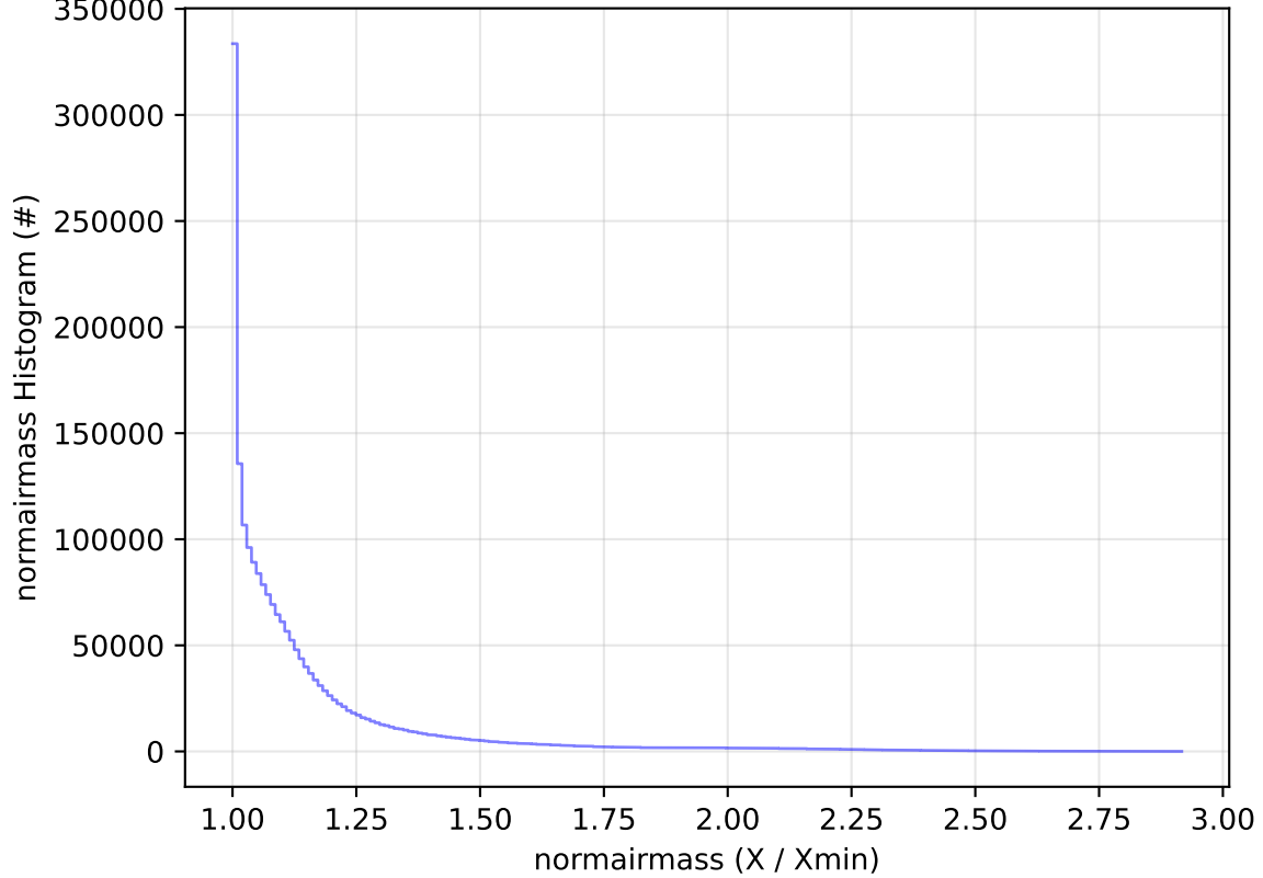
too_elab_2yr_r128_d3_ugrizy_v3.4_10yrs All sky all bands: normairmass Histogram
