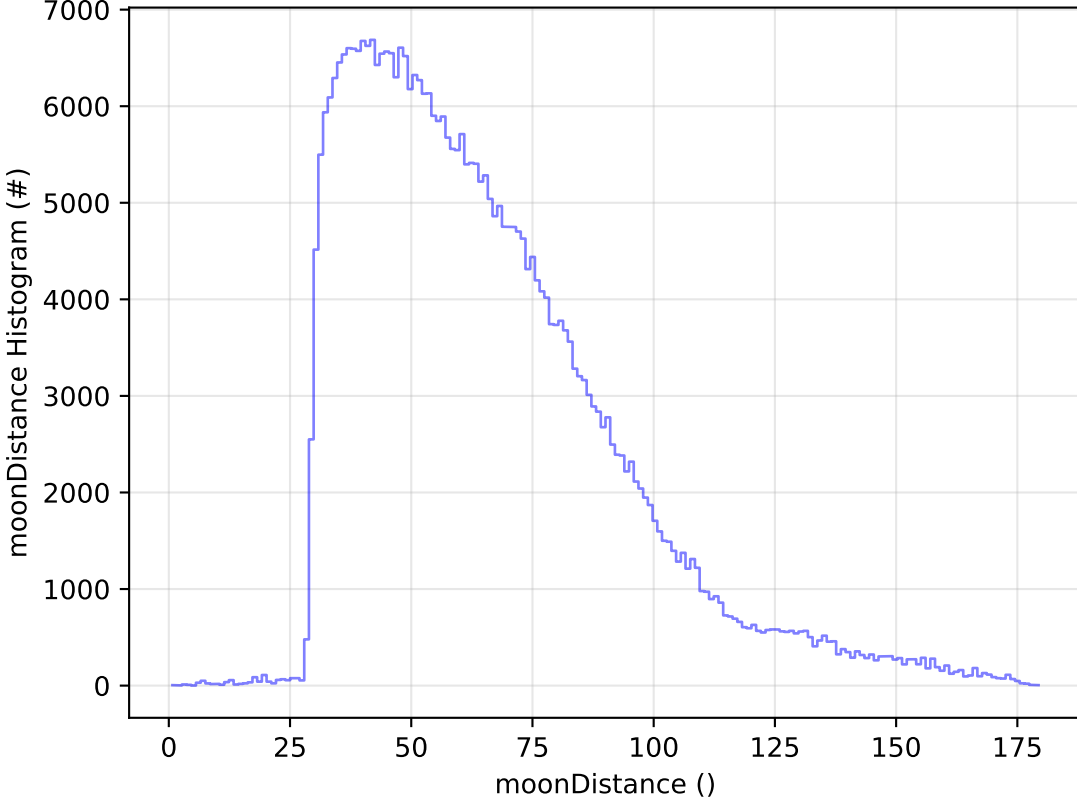
too_elab_2yr_r128_d3_ugrizy_v3.4_10yrs WFD y band: moonDistance Histogram
