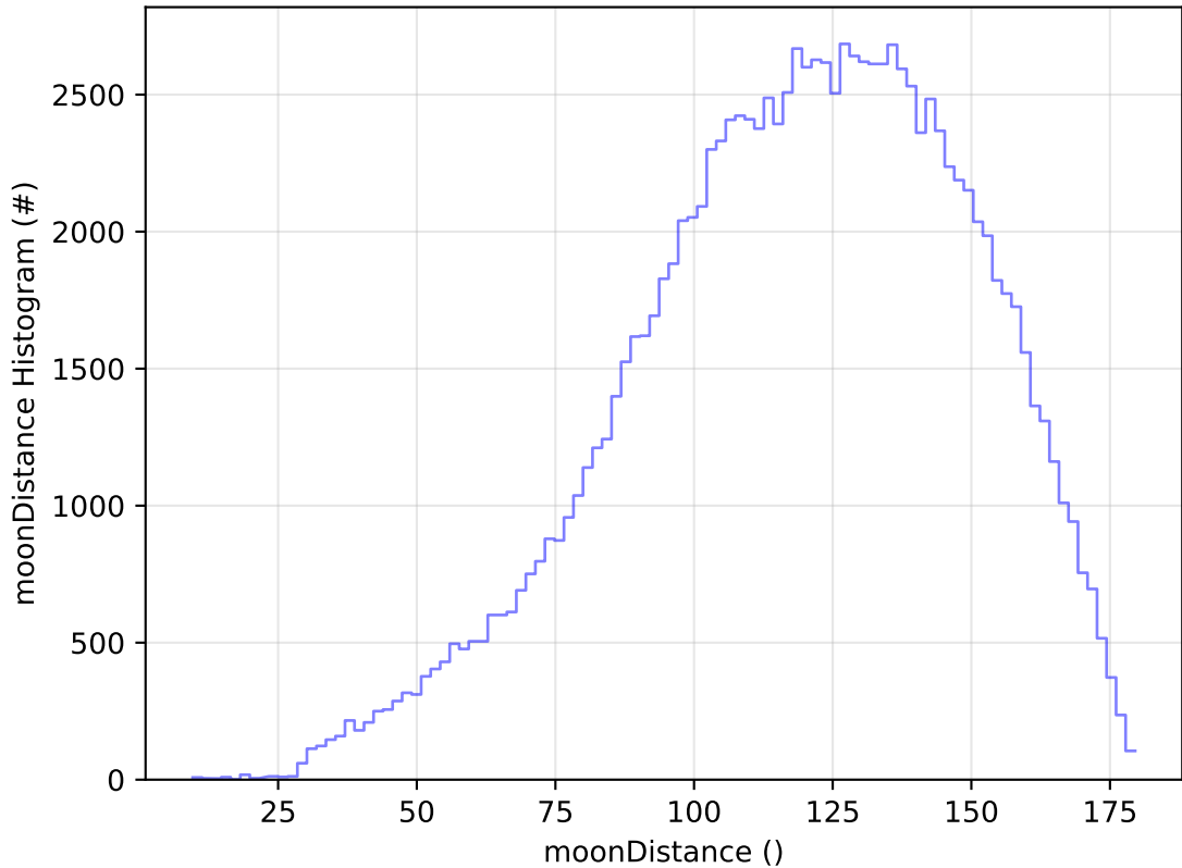
too_elab_2yr_r128_d3_ugrizy_v3.4_10yrs WFD u band: moonDistance Histogram
