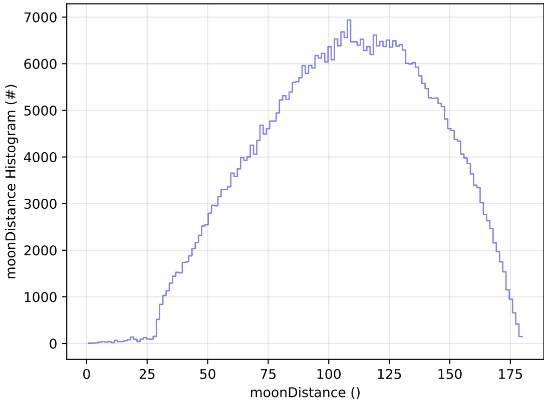
too_elab_2yr_r128_d3_ugrizy_v3.4_10yrs WFD r band: moonDistance Histogram
