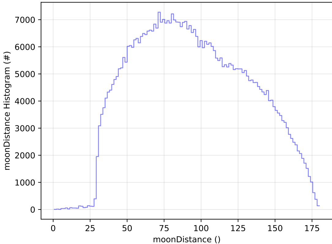
too_elab_2yr_r128_d3_ugrizy_v3.4_10yrs WFD i band: moonDistance Histogram
