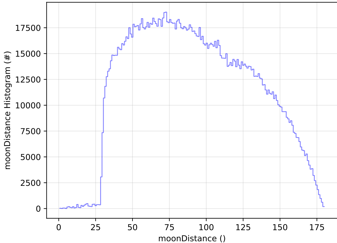
too_elab_2yr_r128_d3_ugrizy_v3.4_10yrs WFD all bands: moonDistance Histogram
