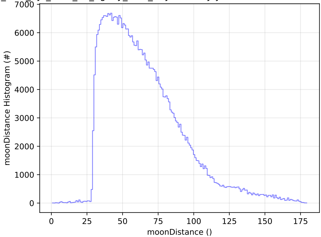
too_elab_2yr_r128_d3_ugrizy_v3.4_10yrs All sky y band: moonDistance Histogram
