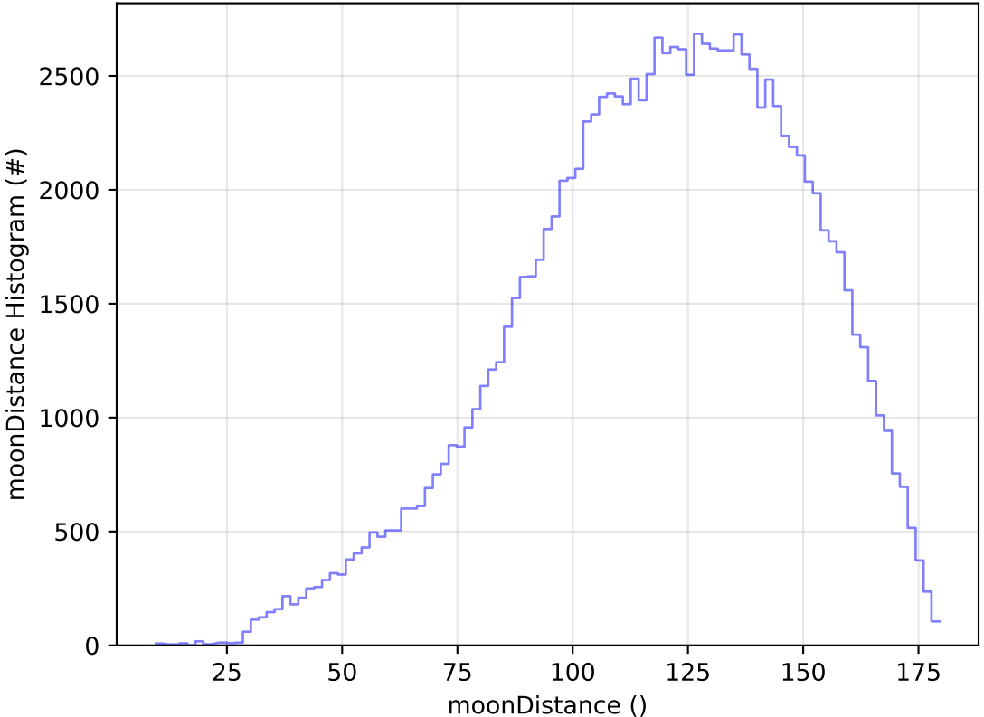
too_elab_2yr_r128_d3_ugrizy_v3.4_10yrs All sky u band: moonDistance Histogram
