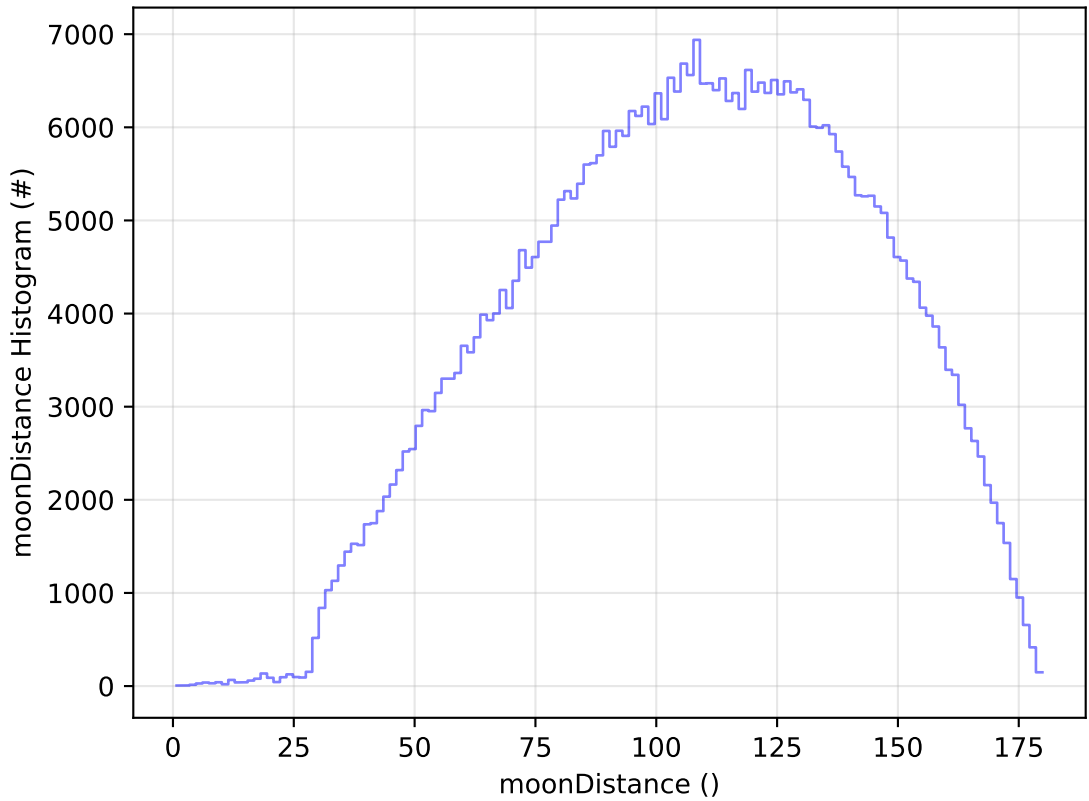
too_elab_2yr_r128_d3_ugrizy_v3.4_10yrs All sky r band: moonDistance Histogram
