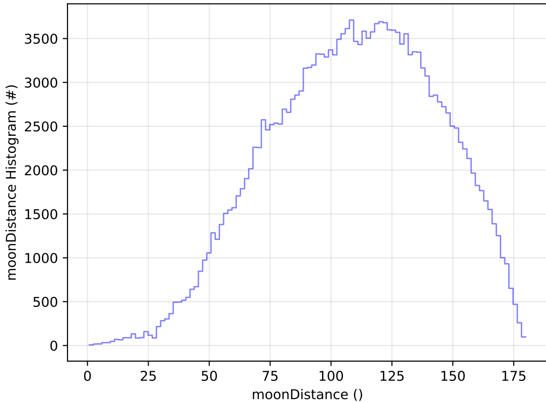
too_elab_2yr_r128_d3_ugrizy_v3.4_10yrs All sky g band: moonDistance Histogram
