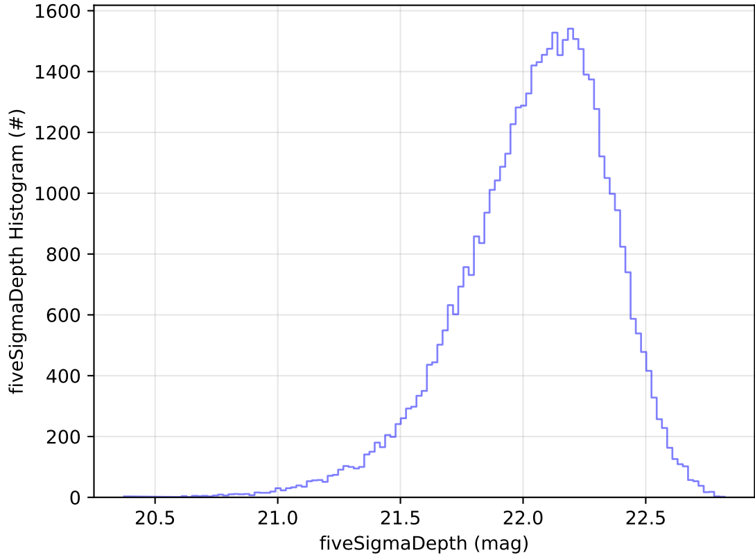
too_elab_2yr_r128_d3_ugrizy_v3.4_10yrs Yr 1 y band: fiveSigmaDepth Histogram
