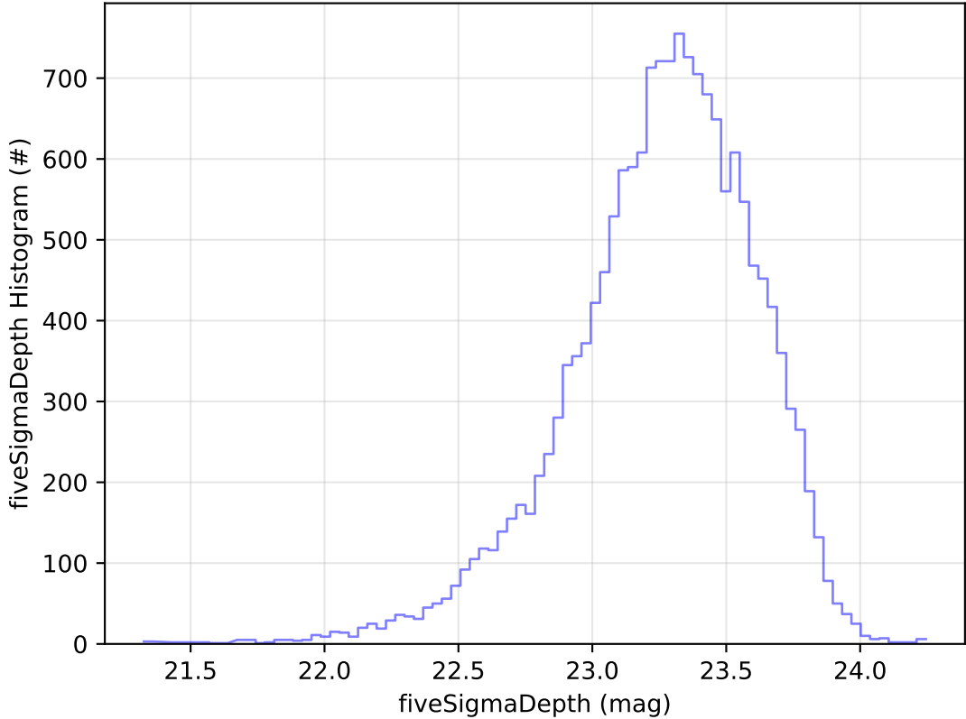
too_elab_2yr_r128_d3_ugrizy_v3.4_10yrs Yr 1 u band: fiveSigmaDepth Histogram
