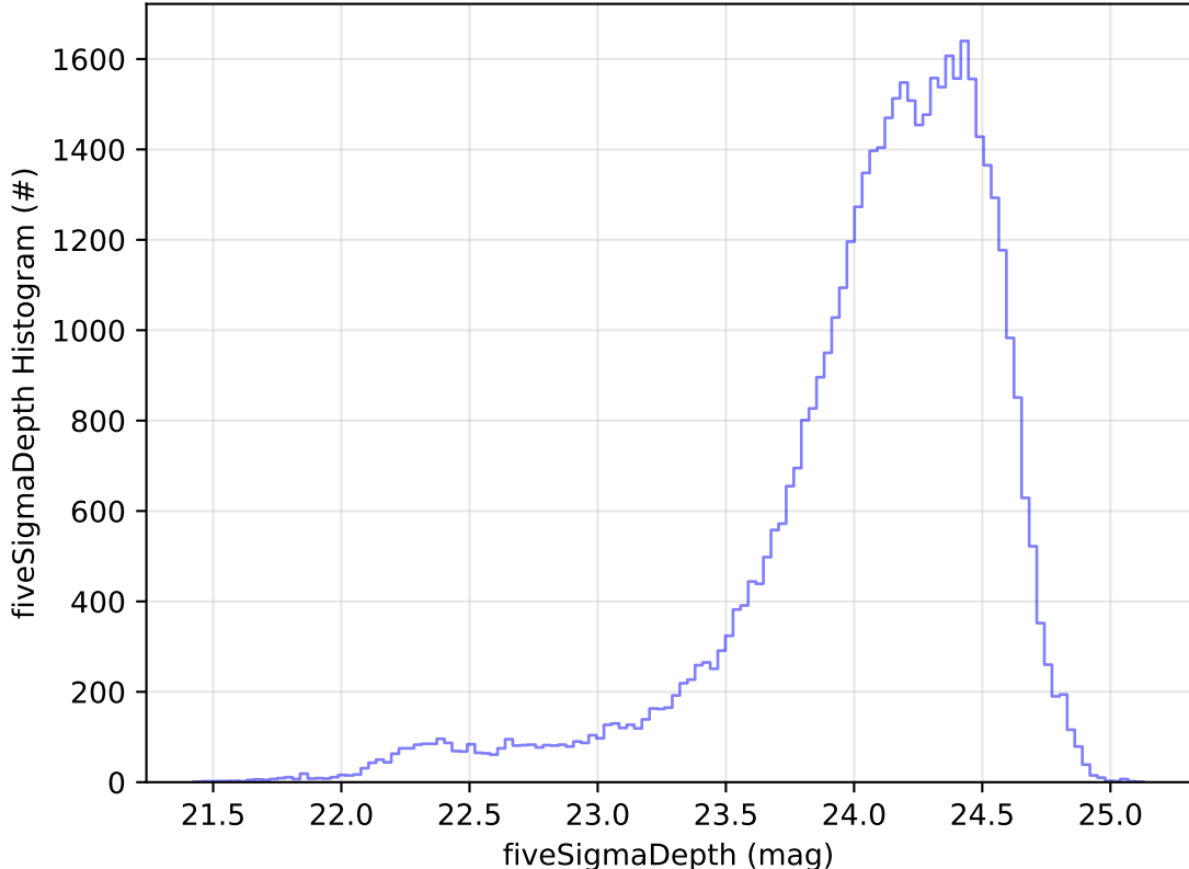
too_elab_2yr_r128_d3_ugrizy_v3.4_10yrs Yr 1 r band: fiveSigmaDepth Histogram
