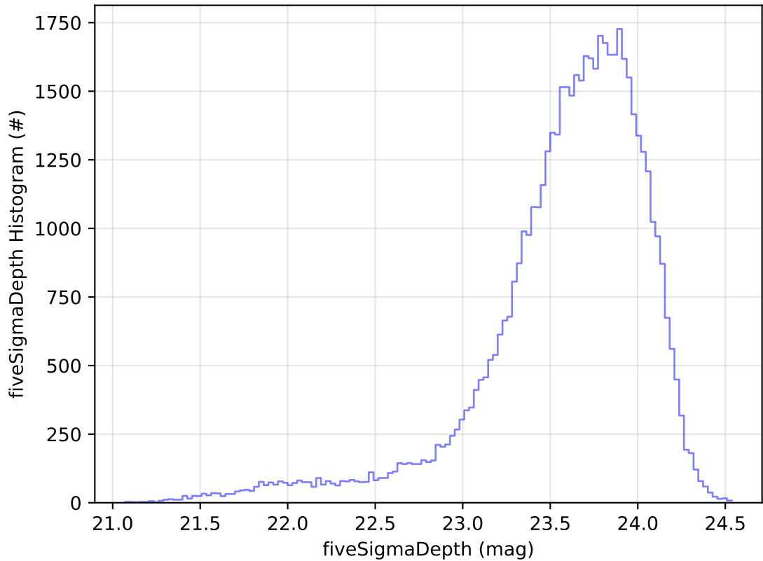
too_elab_2yr_r128_d3_ugrizy_v3.4_10yrs Yr 1 i band: fiveSigmaDepth Histogram
