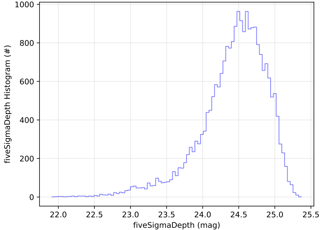
too_elab_2yr_r128_d3_ugrizy_v3.4_10yrs Yr 1 g band: fiveSigmaDepth Histogram
