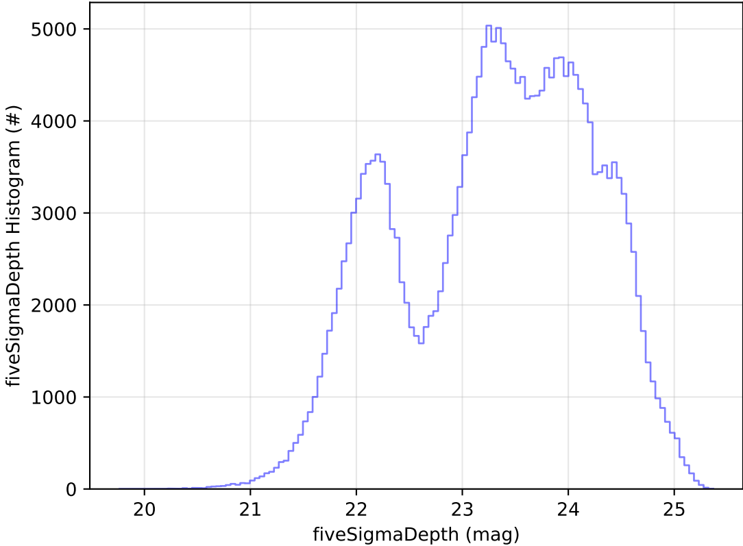
too_elab_2yr_r128_d3_ugrizy_v3.4_10yrs Yr 1 all bands: fiveSigmaDepth Histogram
