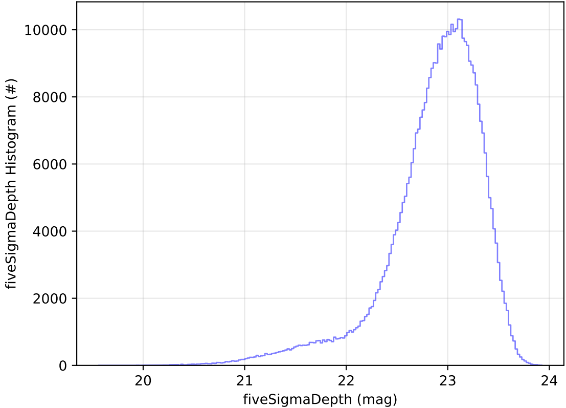
too_elab_2yr_r128_d3_ugrizy_v3.4_10yrs WFD z band: fiveSigmaDepth Histogram
