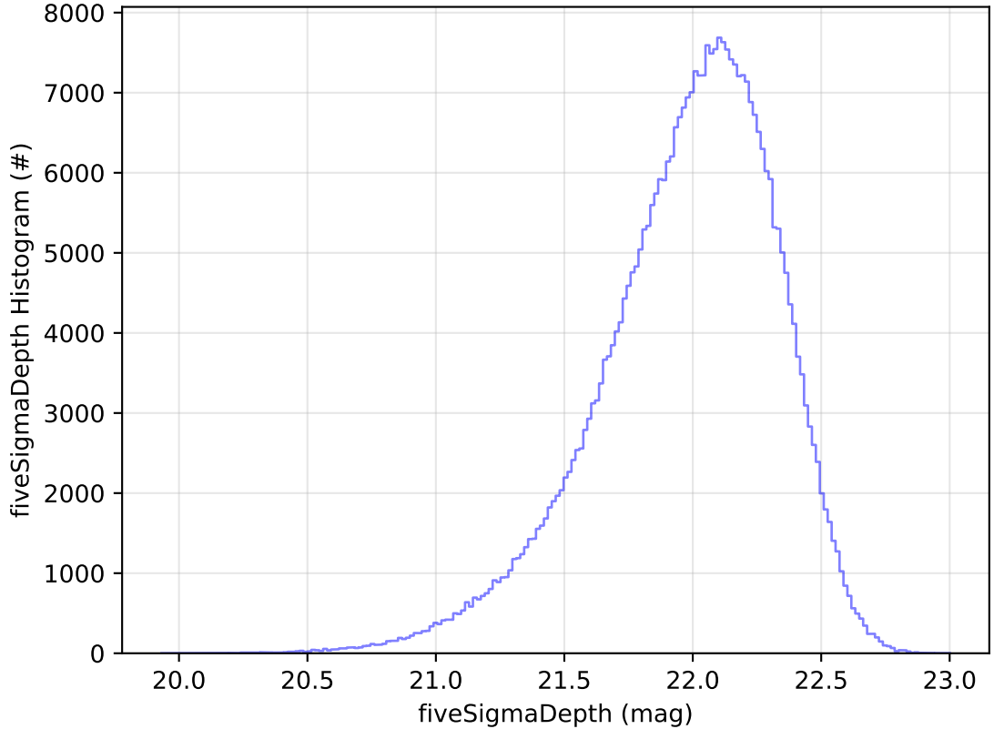
too_elab_2yr_r128_d3_ugrizy_v3.4_10yrs WFD y band: fiveSigmaDepth Histogram
