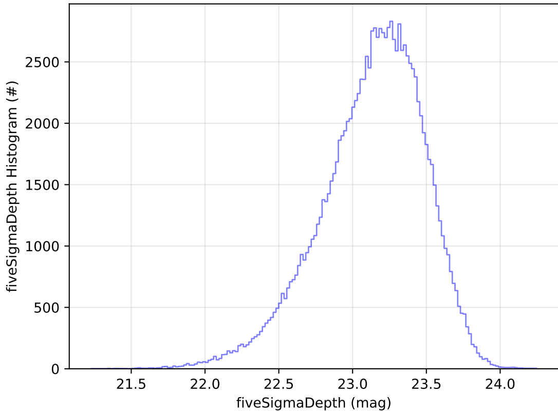
too_elab_2yr_r128_d3_ugrizy_v3.4_10yrs WFD u band: fiveSigmaDepth Histogram
