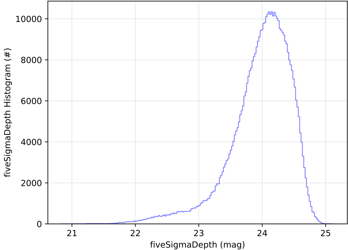
too_elab_2yr_r128_d3_ugrizy_v3.4_10yrs WFD r band: fiveSigmaDepth Histogram
