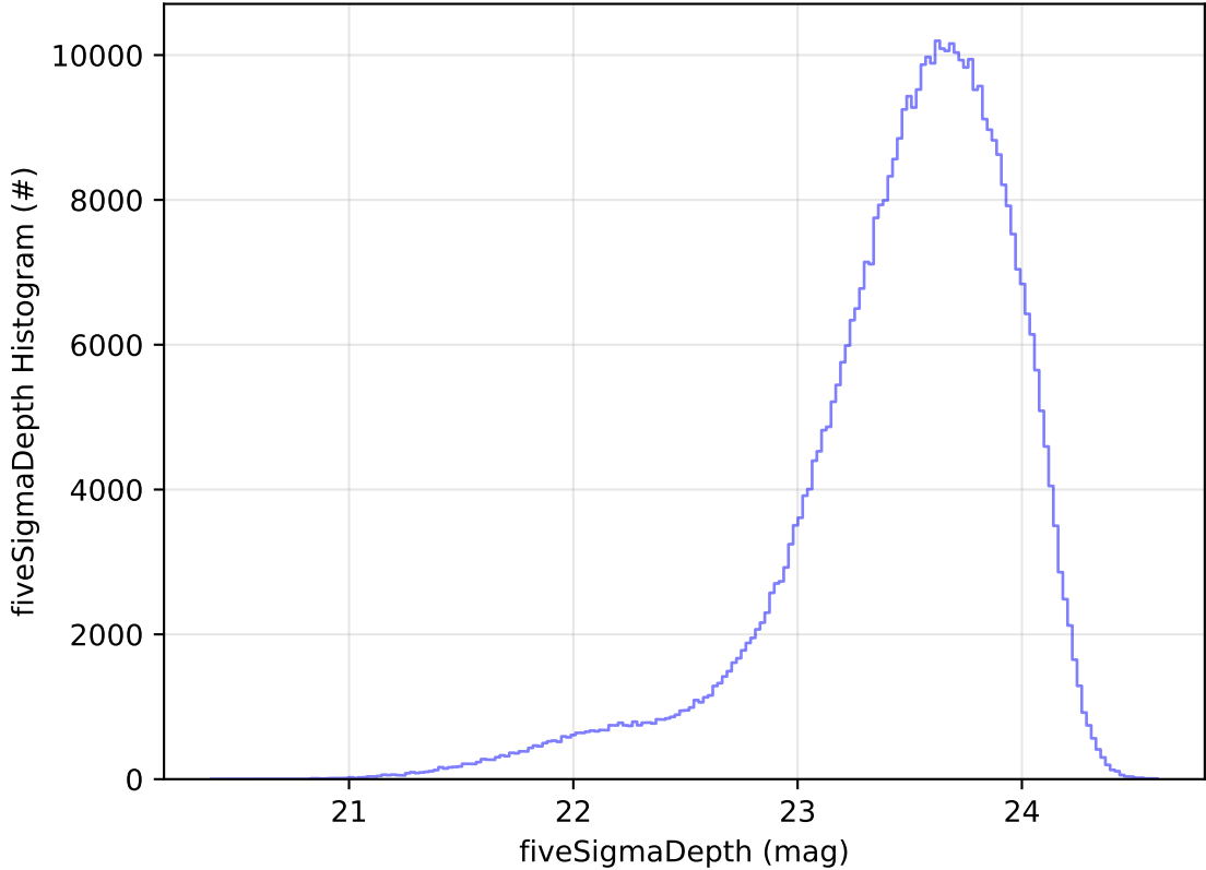
too_elab_2yr_r128_d3_ugrizy_v3.4_10yrs WFD i band: fiveSigmaDepth Histogram
