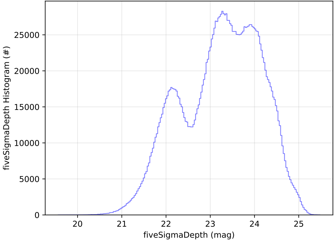
too_elab_2yr_r128_d3_ugrizy_v3.4_10yrs WFD all bands: fiveSigmaDepth Histogram
