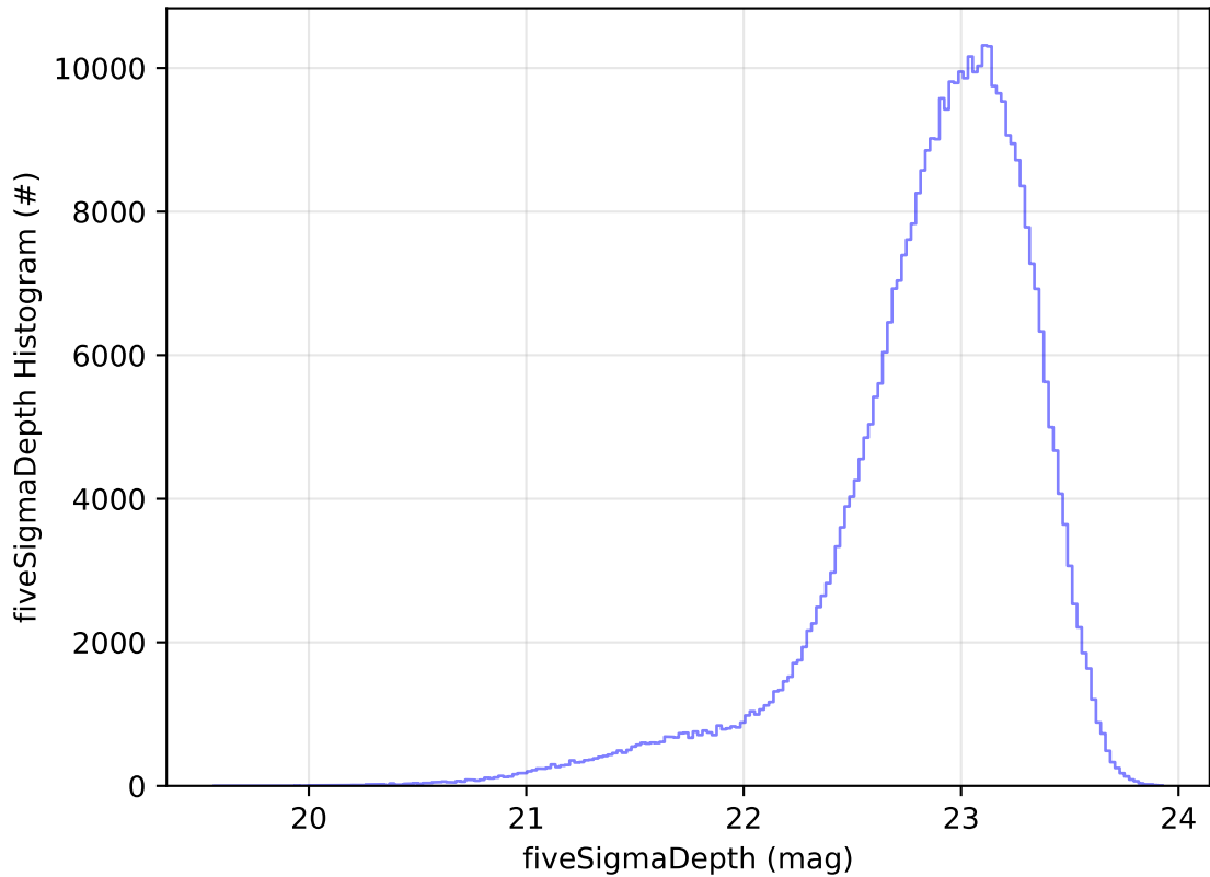
too_elab_2yr_r128_d3_ugrizy_v3.4_10yrs All sky z band: fiveSigmaDepth Histogram
