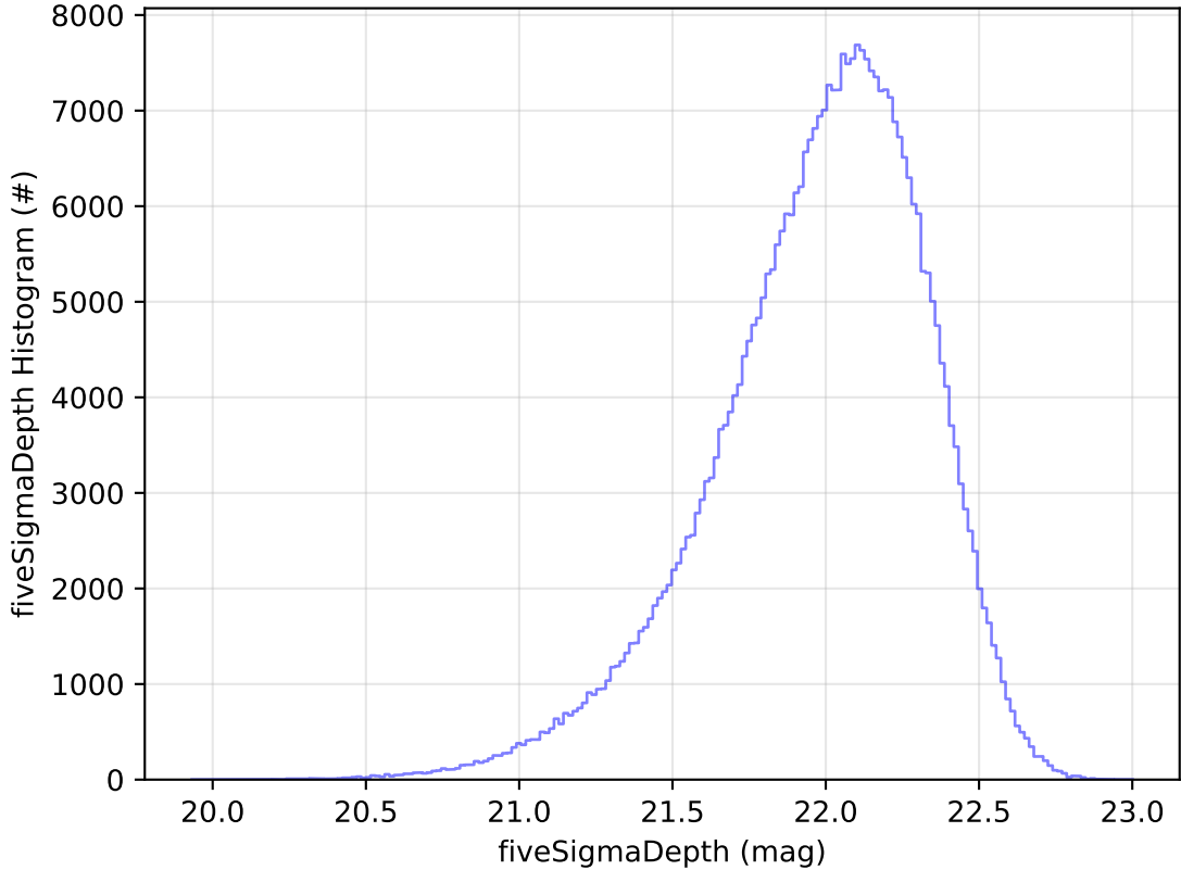
too_elab_2yr_r128_d3_ugrizy_v3.4_10yrs All sky y band: fiveSigmaDepth Histogram
