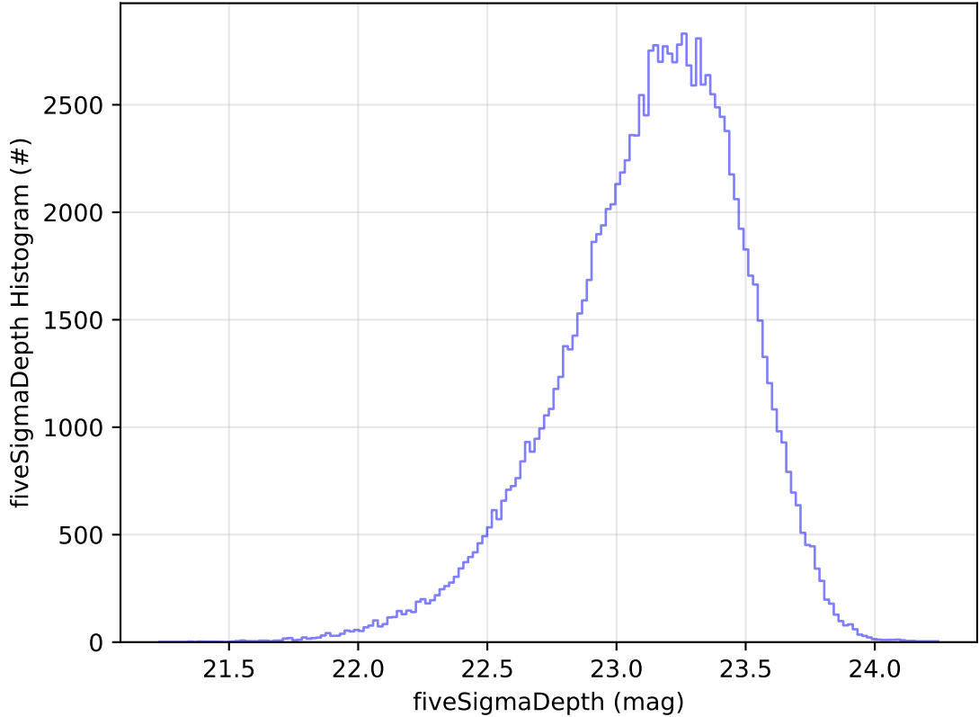
too_elab_2yr_r128_d3_ugrizy_v3.4_10yrs All sky u band: fiveSigmaDepth Histogram
