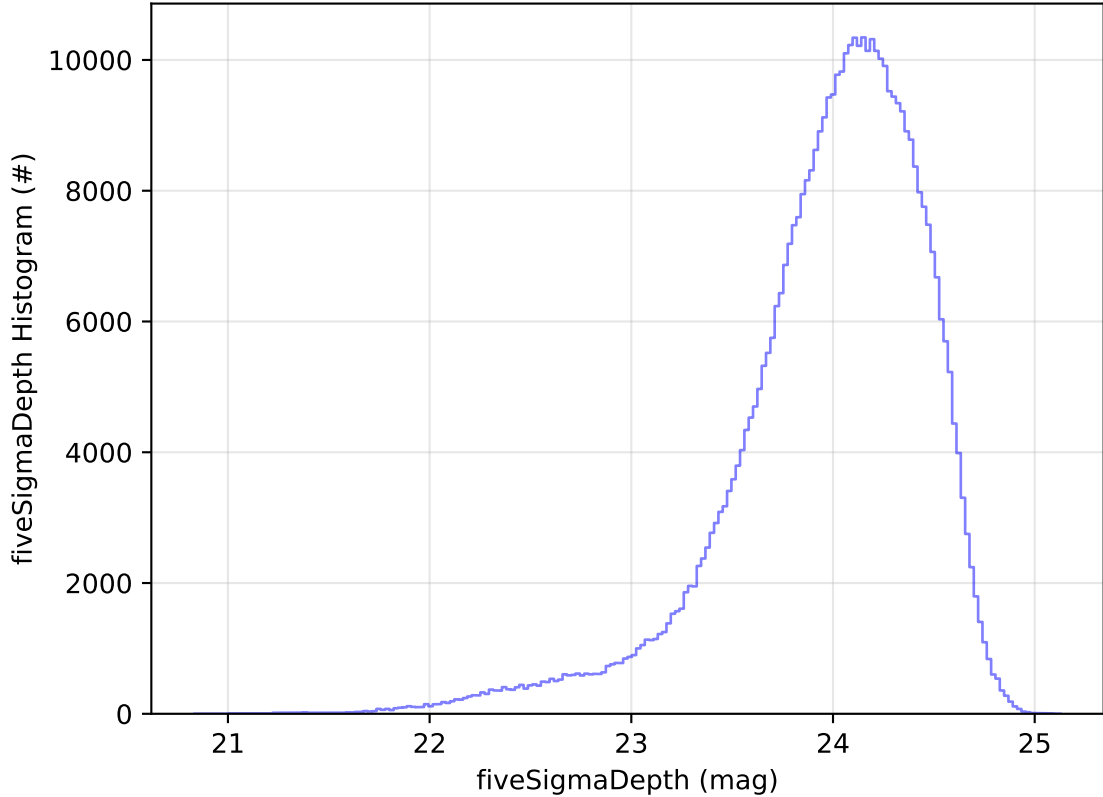
too_elab_2yr_r128_d3_ugrizy_v3.4_10yrs All sky r band: fiveSigmaDepth Histogram
