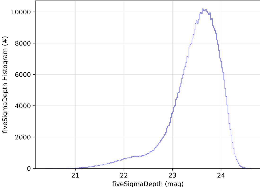
too_elab_2yr_r128_d3_ugrizy_v3.4_10yrs All sky i band: fiveSigmaDepth Histogram
