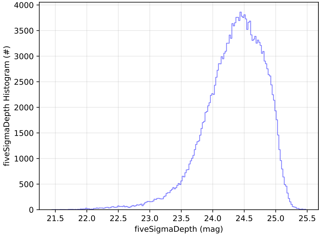
too_elab_2yr_r128_d3_ugrizy_v3.4_10yrs All sky g band: fiveSigmaDepth Histogram
