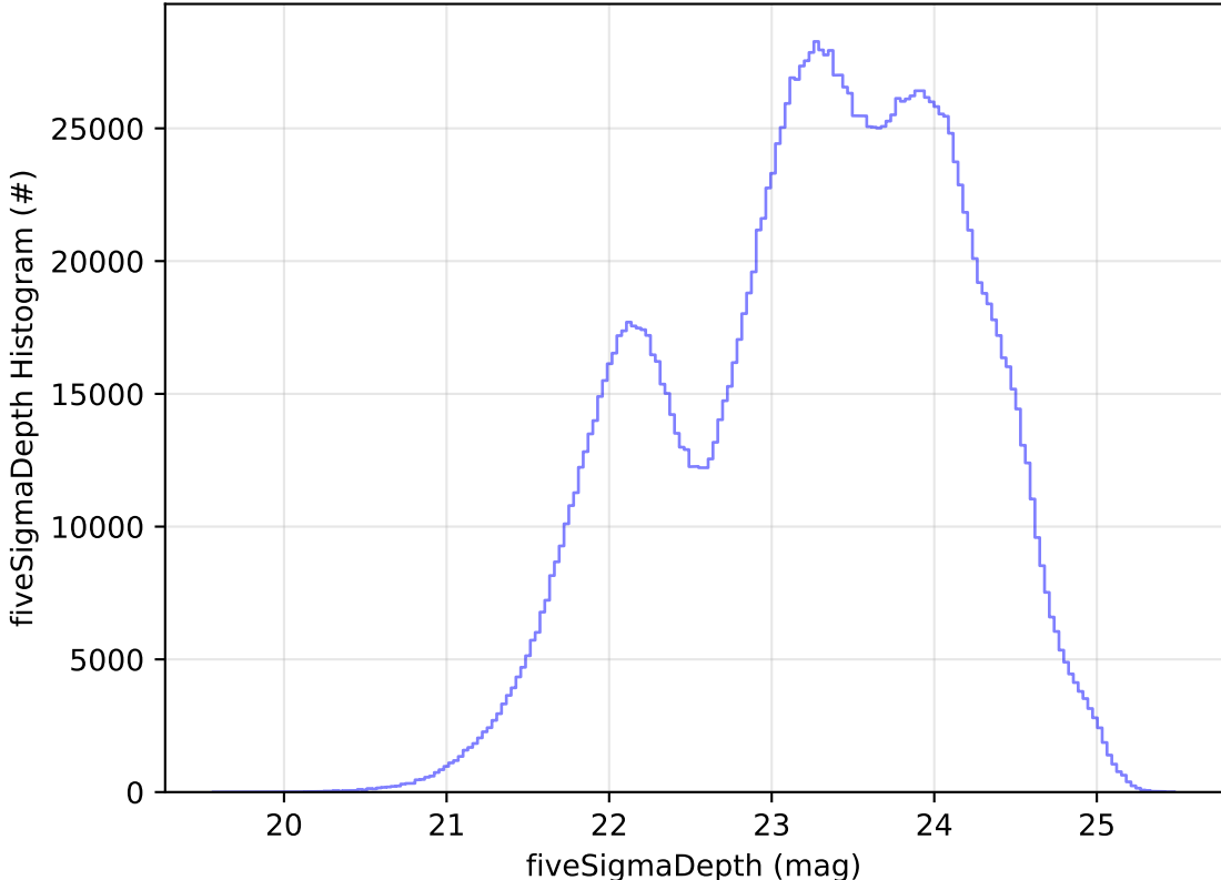
too_elab_2yr_r128_d3_ugrizy_v3.4_10yrs All sky all bands: fiveSigmaDepth Histogram
