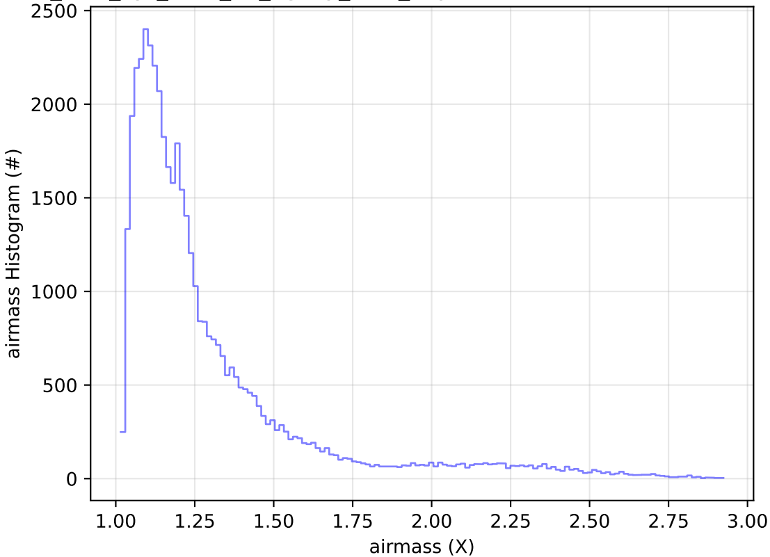
too_elab_2yr_r128_d3_ugrizy_v3.4_10yrs Yr 1 z band: airmass Histogram
