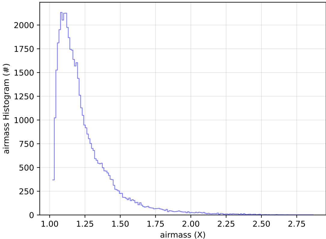
too_elab_2yr_r128_d3_ugrizy_v3.4_10yrs Yr 1 y band: airmass Histogram
