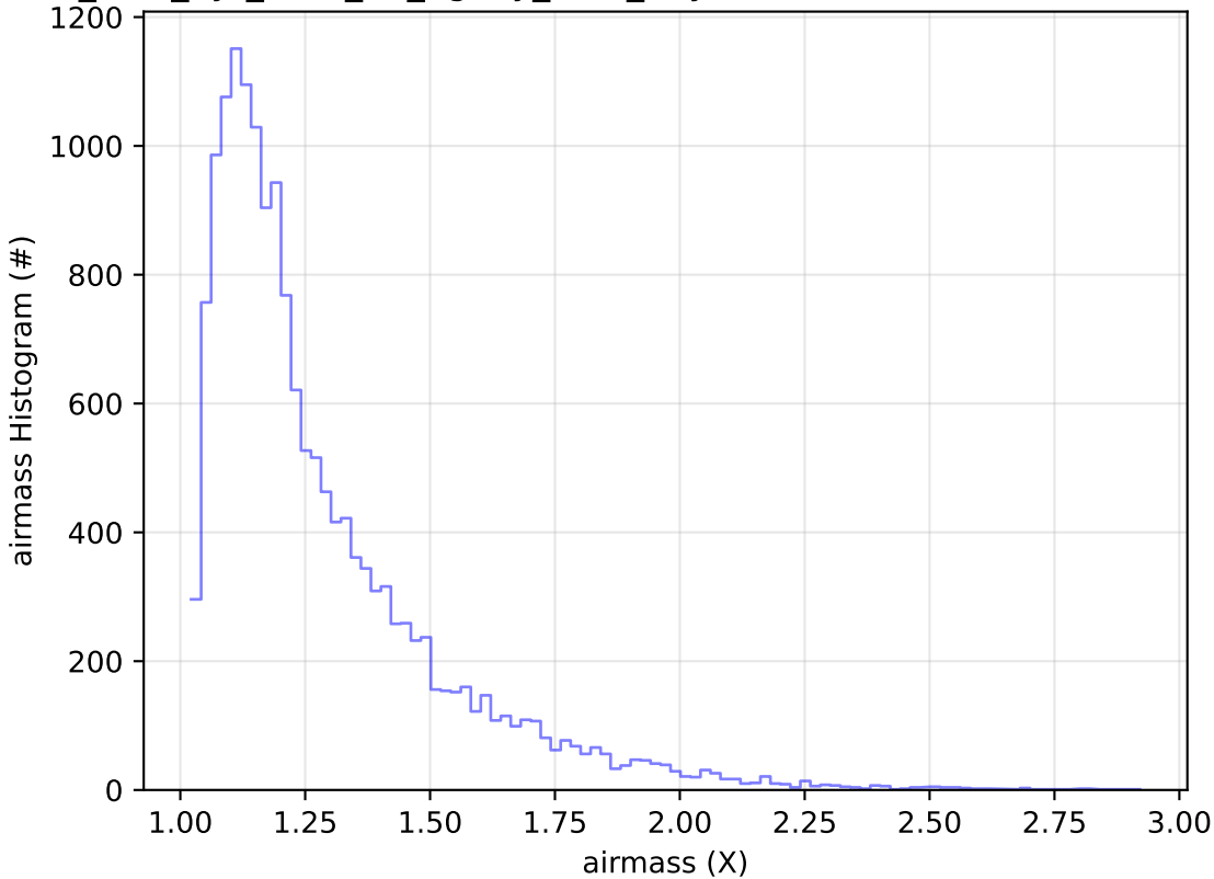
too_elab_2yr_r128_d3_ugrizy_v3.4_10yrs Yr 1 u band: airmass Histogram
