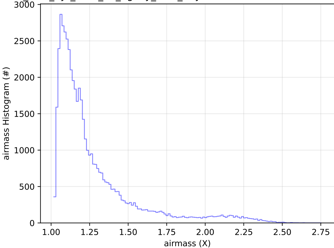
too_elab_2yr_r128_d3_ugrizy_v3.4_10yrs Yr 1 r band: airmass Histogram
