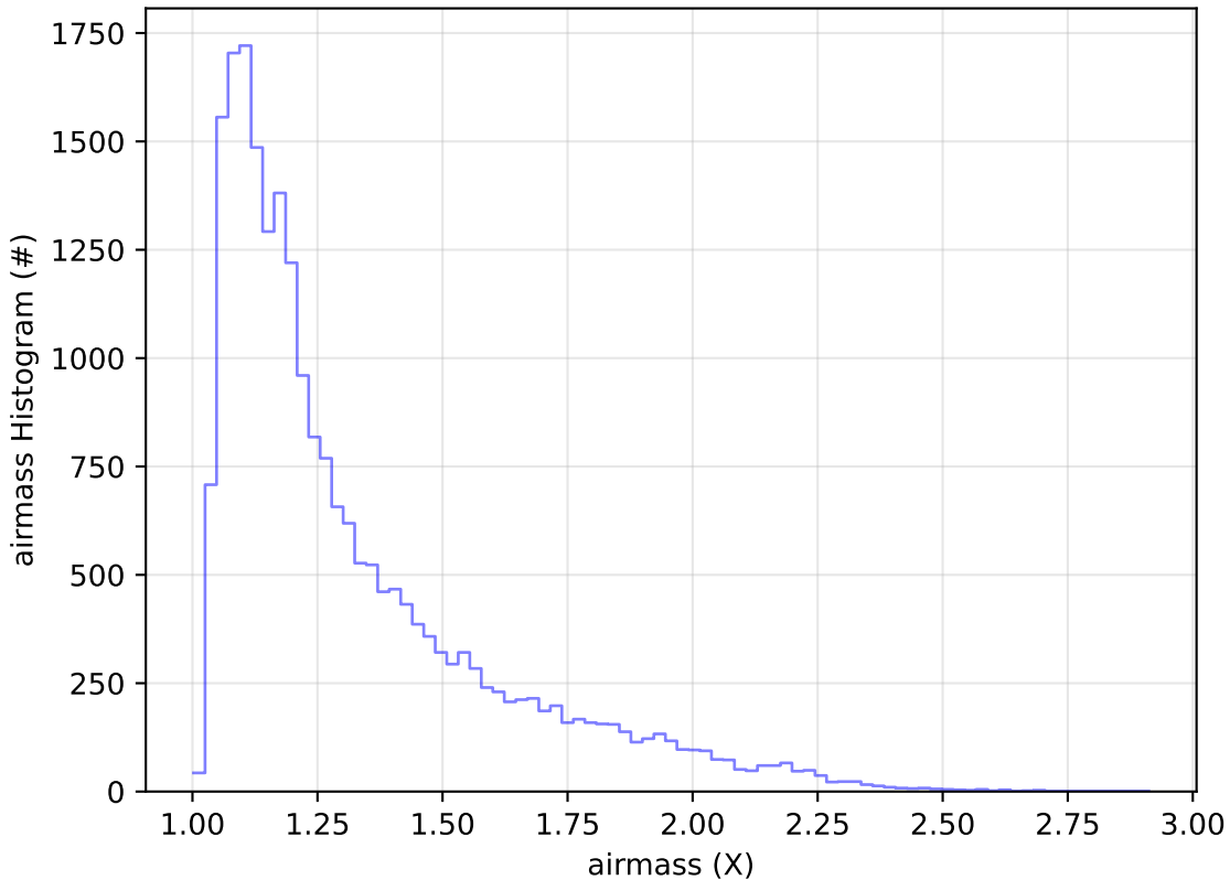
too_elab_2yr_r128_d3_ugrizy_v3.4_10yrs Yr 1 g band: airmass Histogram
