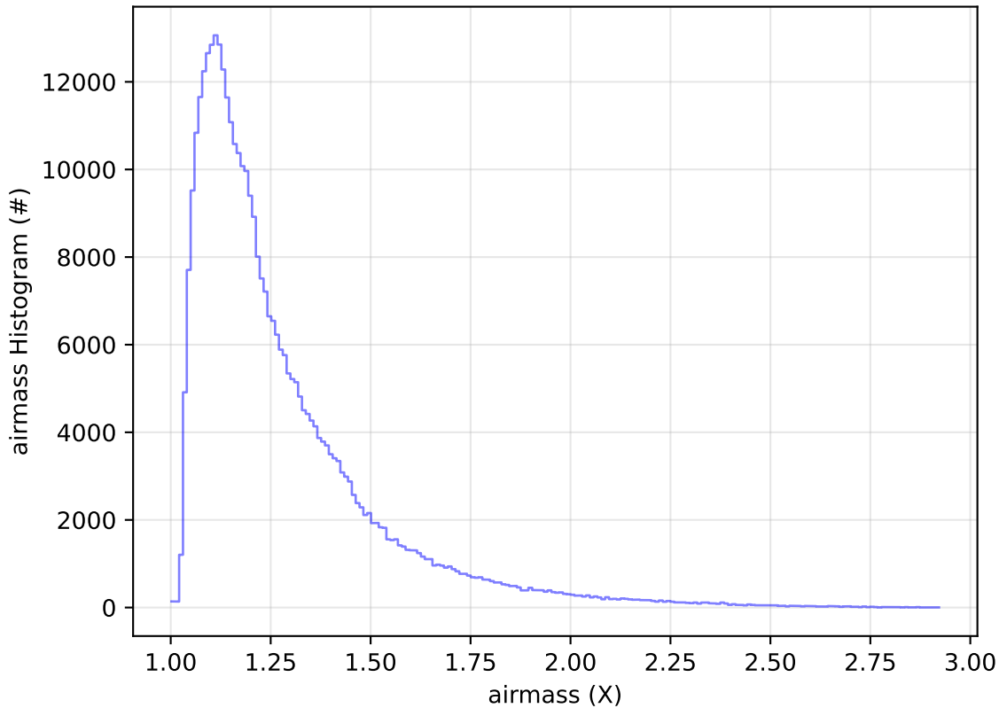
too_elab_2yr_r128_d3_ugrizy_v3.4_10yrs WFD y band: airmass Histogram
