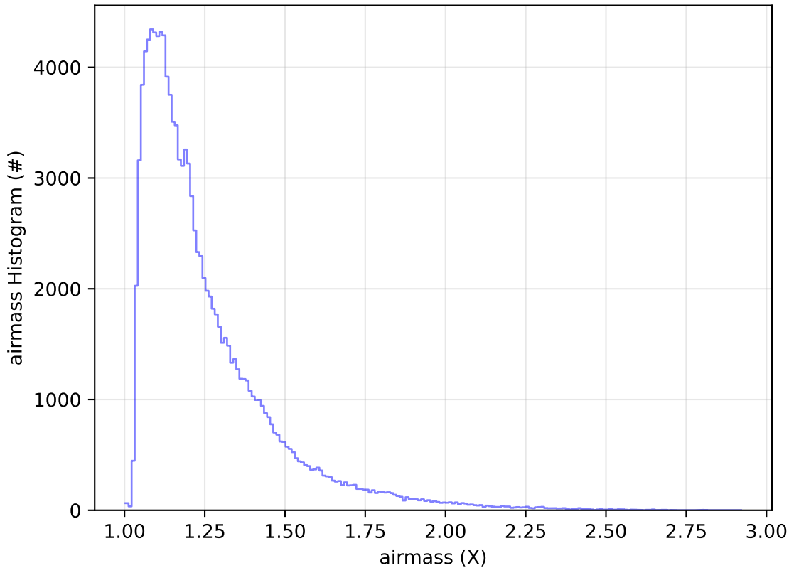
too_elab_2yr_r128_d3_ugrizy_v3.4_10yrs WFD u band: airmass Histogram
