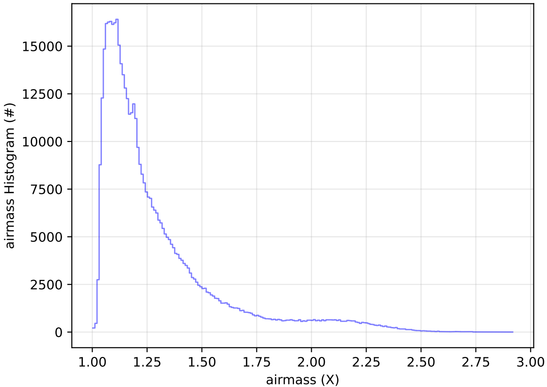
too_elab_2yr_r128_d3_ugrizy_v3.4_10yrs WFD r band: airmass Histogram
