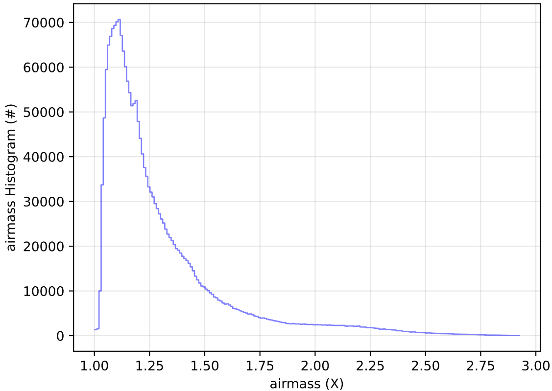
too_elab_2yr_r128_d3_ugrizy_v3.4_10yrs WFD all bands: airmass Histogram
