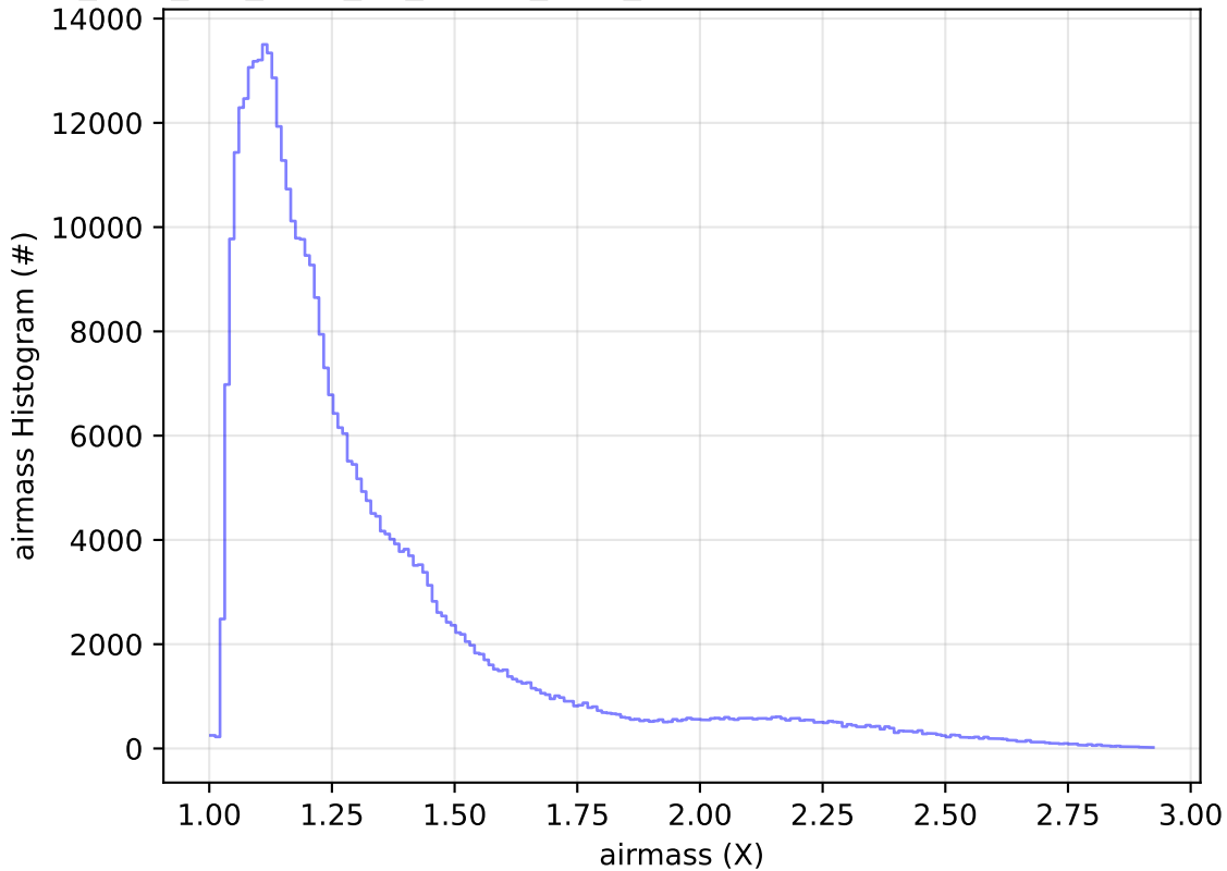
too_elab_2yr_r128_d3_ugrizy_v3.4_10yrs All sky z band: airmass Histogram
