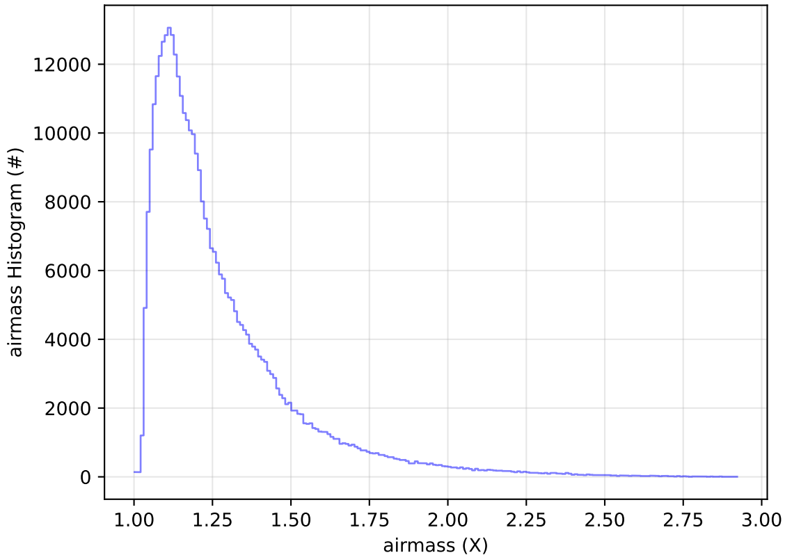
too_elab_2yr_r128_d3_ugrizy_v3.4_10yrs All sky y band: airmass Histogram
