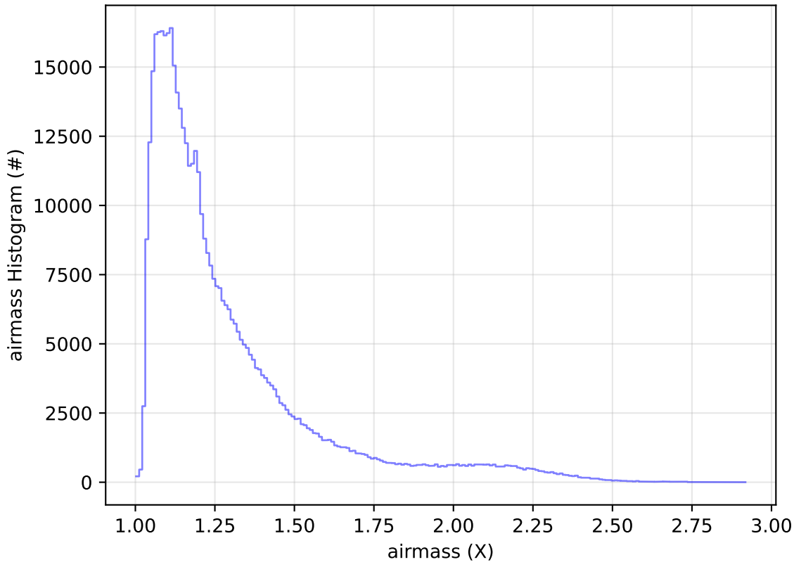
too_elab_2yr_r128_d3_ugrizy_v3.4_10yrs All sky r band: airmass Histogram
