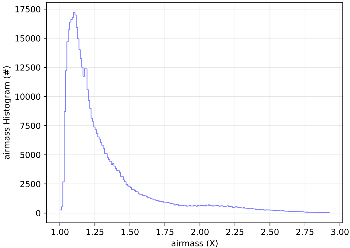
too_elab_2yr_r128_d3_ugrizy_v3.4_10yrs All sky i band: airmass Histogram
