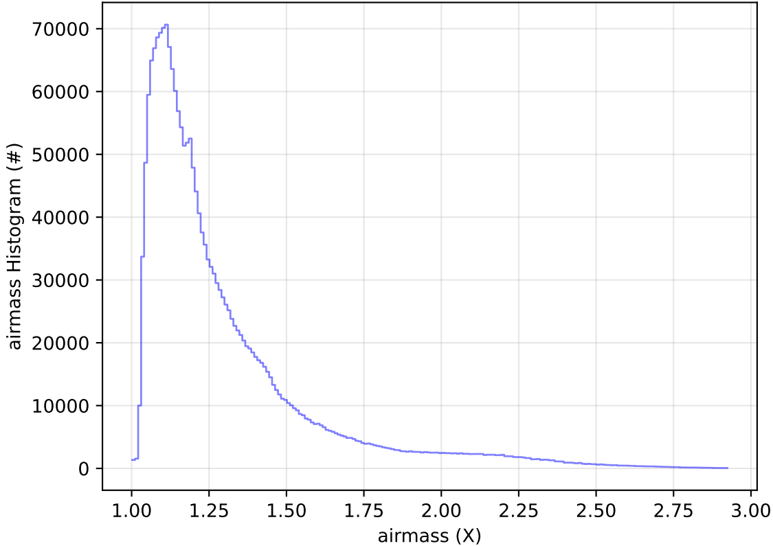
too_elab_2yr_r128_d3_ugrizy_v3.4_10yrs All sky all bands: airmass Histogram
