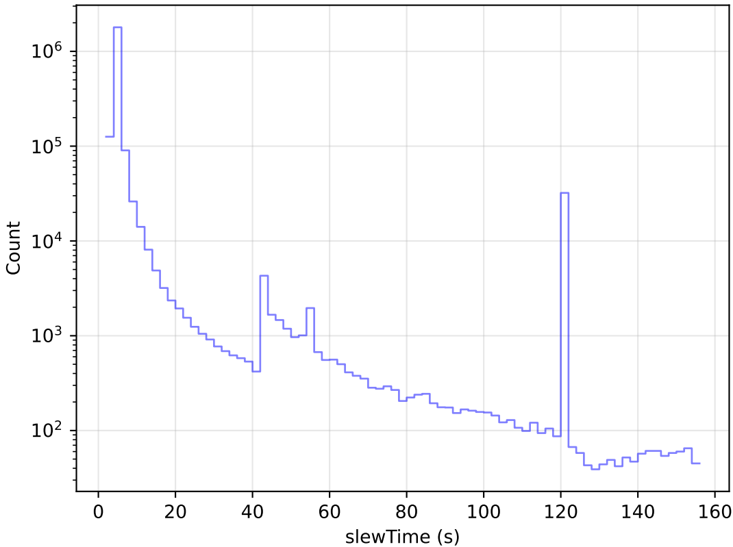
too_elab_2yr_r128_d3_ugrizy_v3.4_10yrs All visits: Slew Time Histogram
