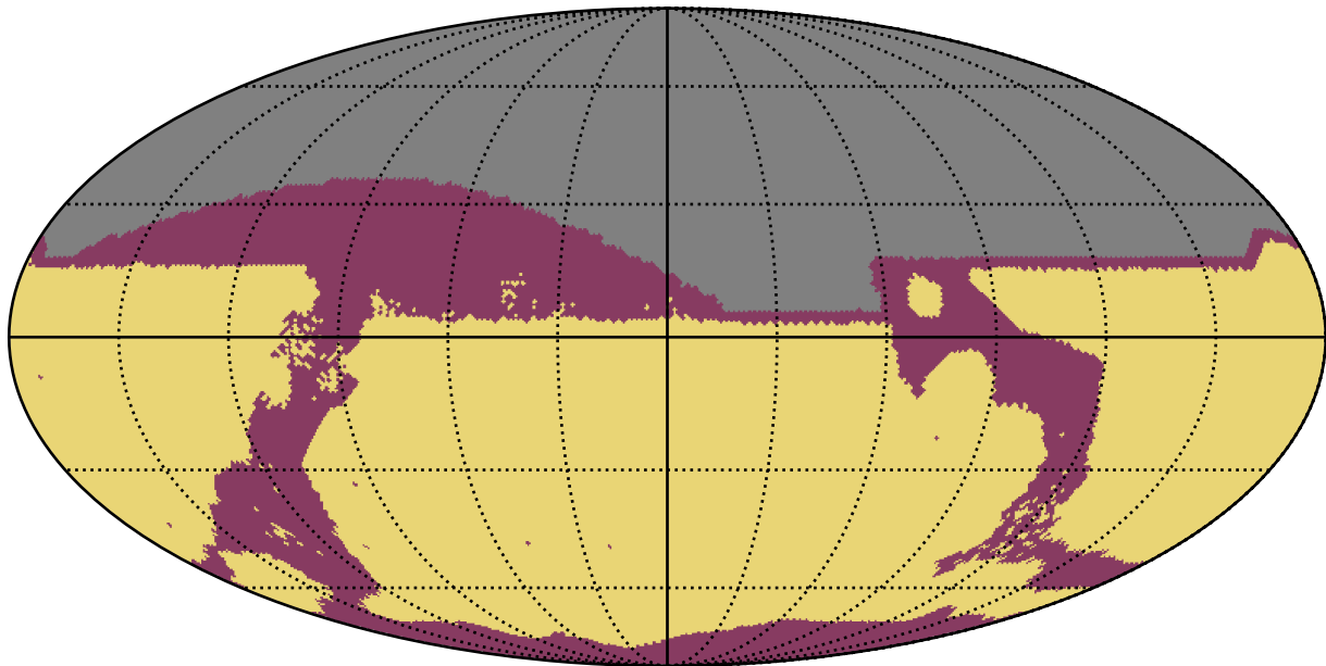
too_elab_2yr_r128_d3_ugrizy_v3.4_10yrs All sky: RapidRevisits
