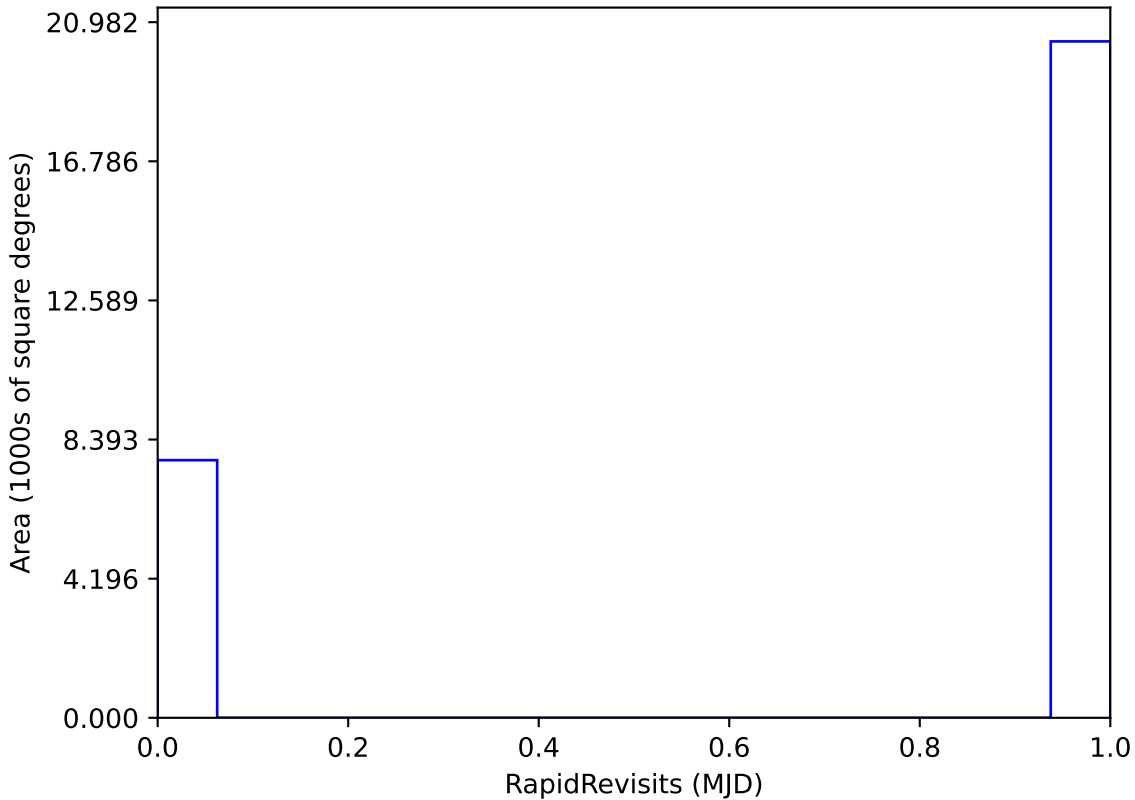
too_elab_2yr_r128_d3_ugrizy_v3.4_10yrs All sky: RapidRevisits
