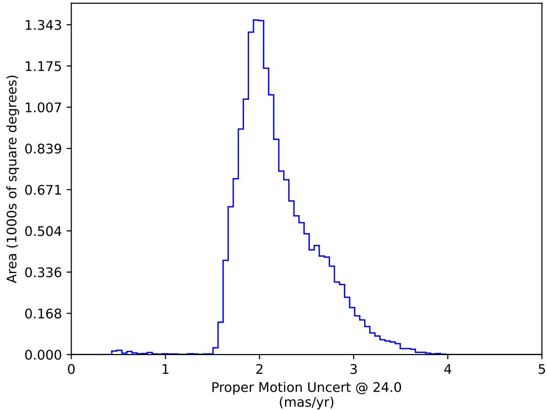
too_elab_2yr_r128_d3_ugrizy_v3.4_10yrs WFD: Proper Motion Uncert @ 24.0
