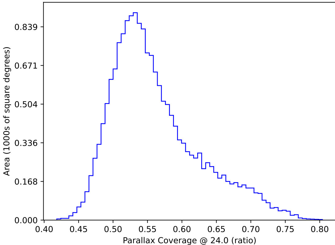
too_elab_2yr_r128_d3_ugrizy_v3.4_10yrs WFD: Parallax Coverage @ 24.0
