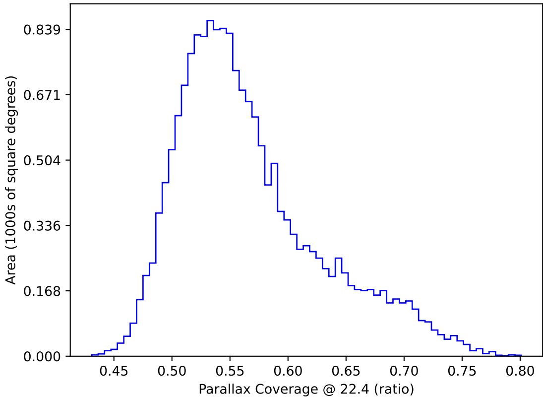
too_elab_2yr_r128_d3_ugrizy_v3.4_10yrs WFD: Parallax Coverage @ 22.4
